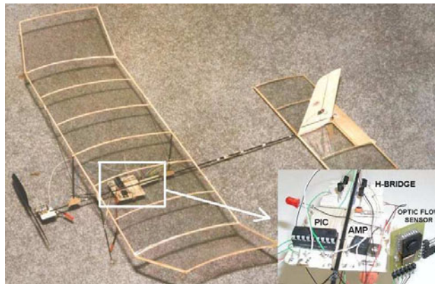
Figure 7: Fixed-wing aircraft equipped with optic flow sensor suite.
