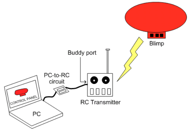
Figure 4: A PC-to-RC circuit converts digital commands to RC signals. Commands are then sent wirelessly to the blimp through a RC transmitter.
