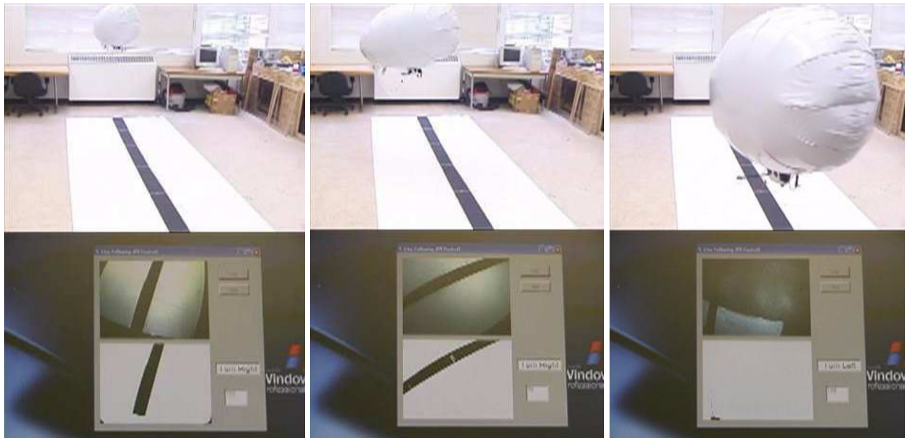
Figure 8: A wireless camera is coupled with a computer vision algorithm to achieve line following.
