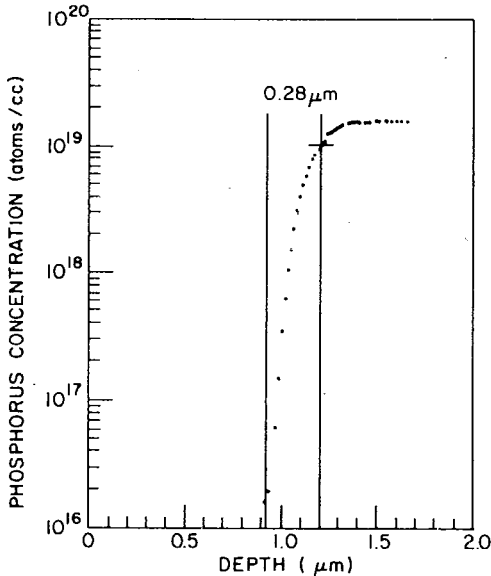
Fig. 13—Impurity concentration profile in transition region.
