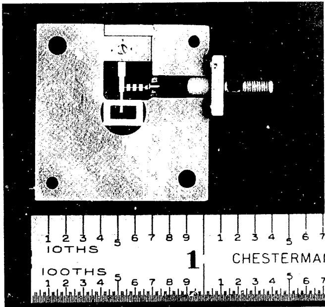
Fig. 22—Millimeter wave hybrid-monolithic circuit on silicon.
