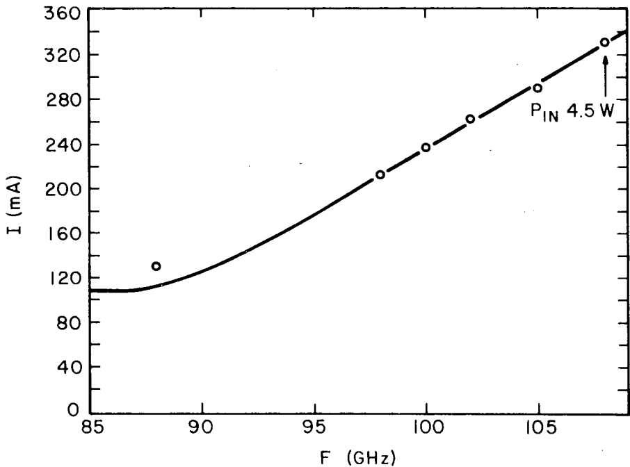
Fig. 20—DC supply current versus IMPATT frequency.
