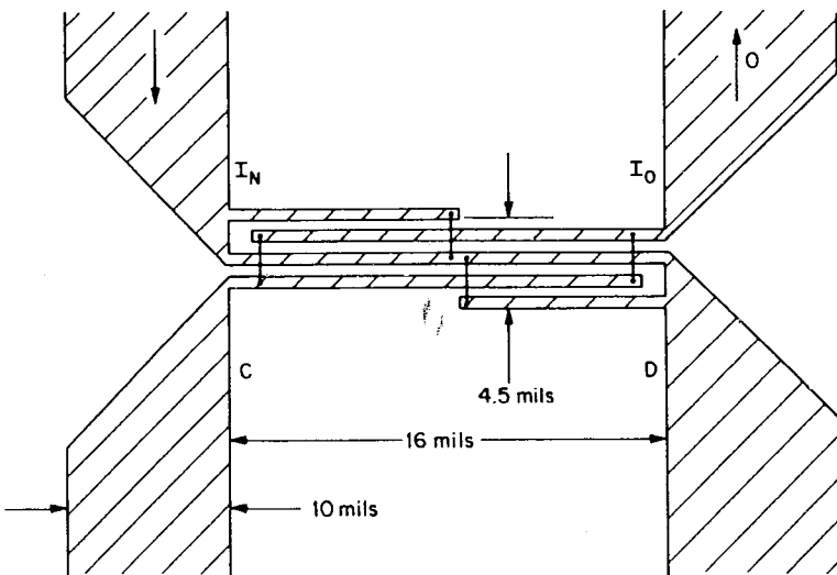
Fig. 7—A Lange coupler for 60-GHz applications.
