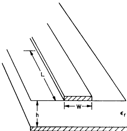
Fig. 8—Dimensions of a microstrip line.
