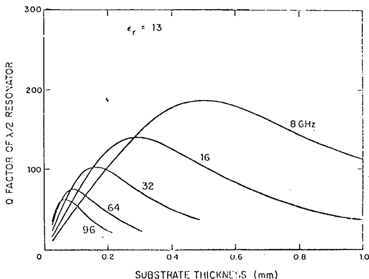
Fig. 5—Q factor versus substrate thickness for 50- \Omega transmission lines. Reprinted from Gopinath 9 (Fig. 3e of Ref. [9], IEEE 1981).
